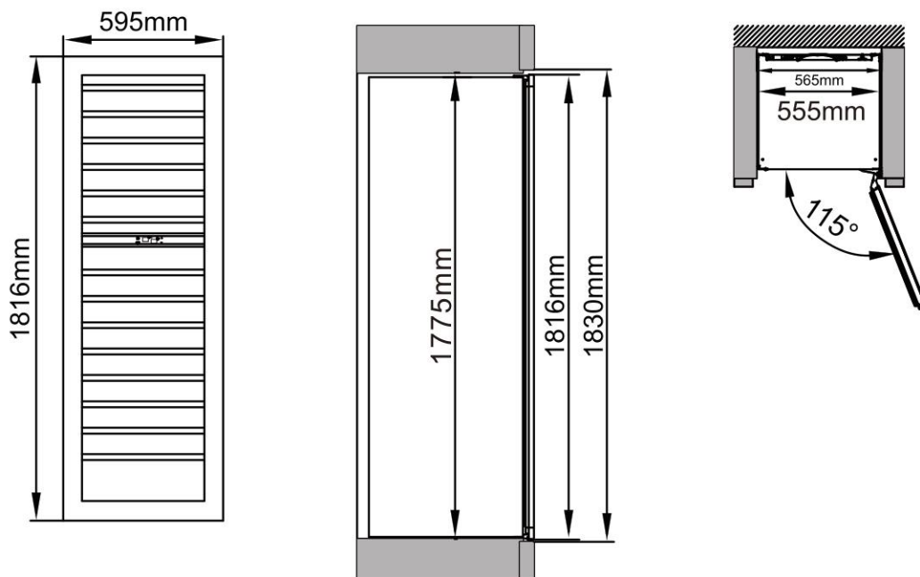
Dimensions — front, side & top
