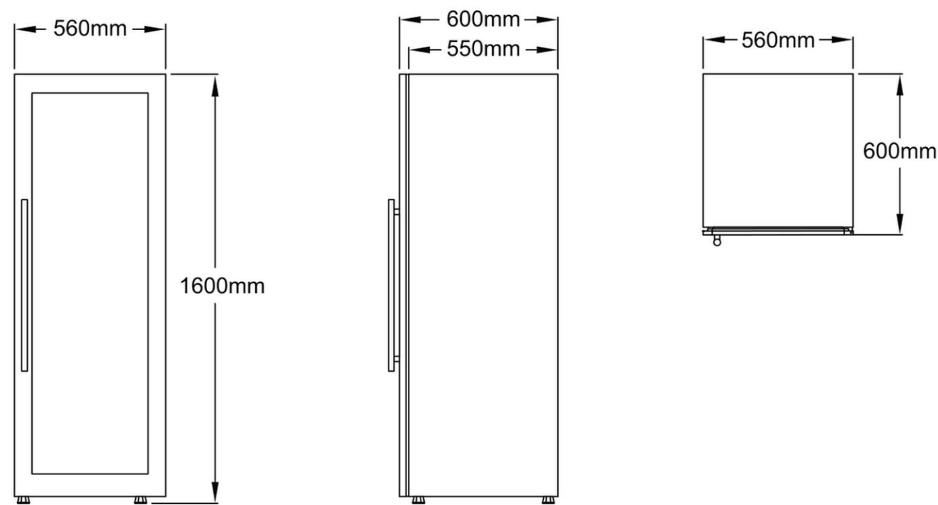
Dimensions — front, side & top
