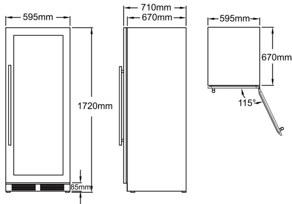
Dimensions — front, side & top
