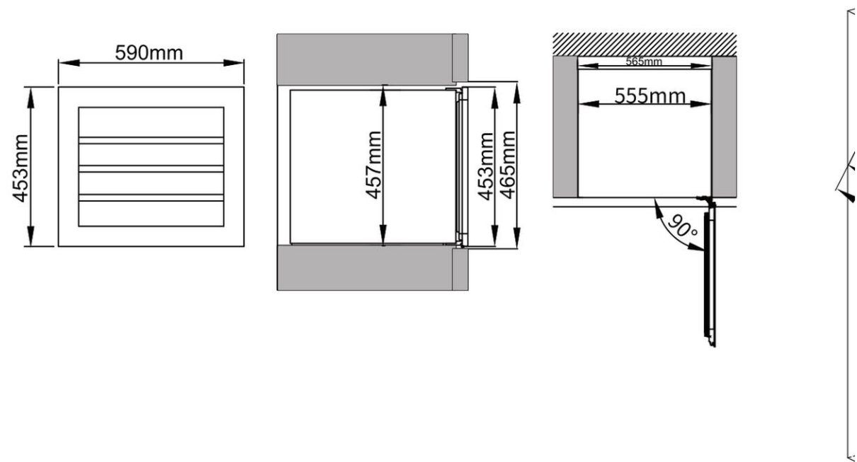
Dimensions — front, side & top
