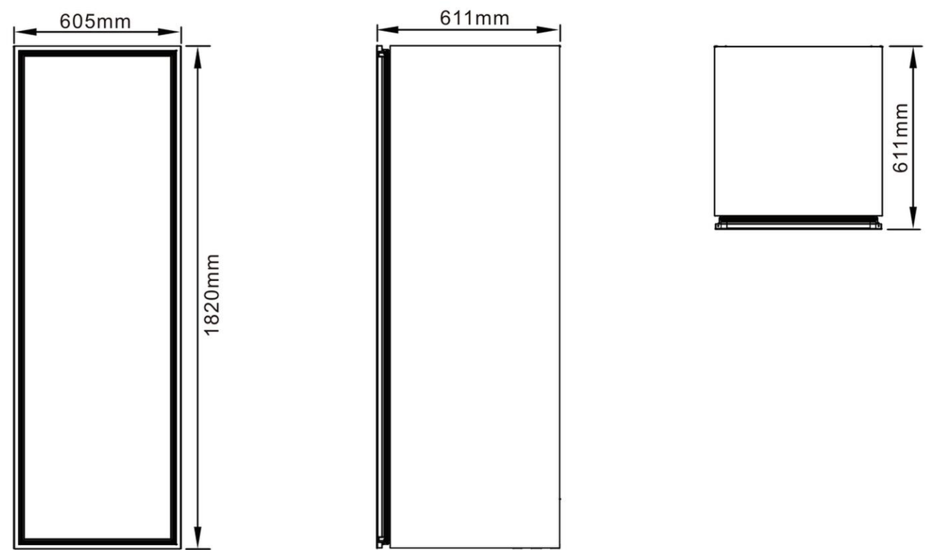
Dimensions — front, side & top
