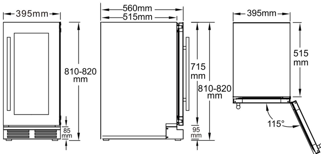
Dimensions — front, side & top
