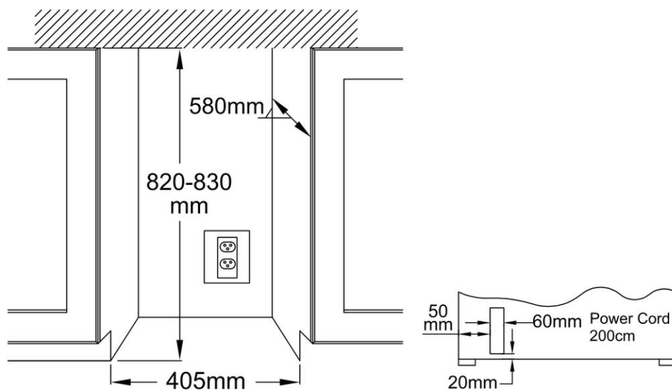
Cabinet Cut-Out
