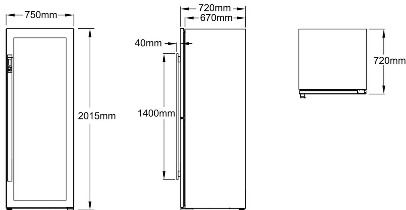
Dimensions — front, side & top
