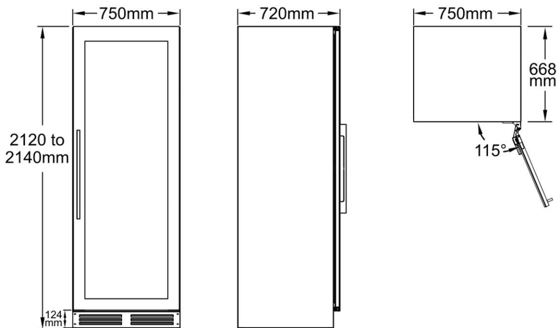
Dimensions — front, side & top
