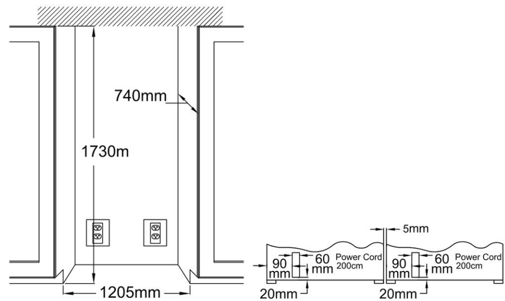
Cabinet Cut-Out
