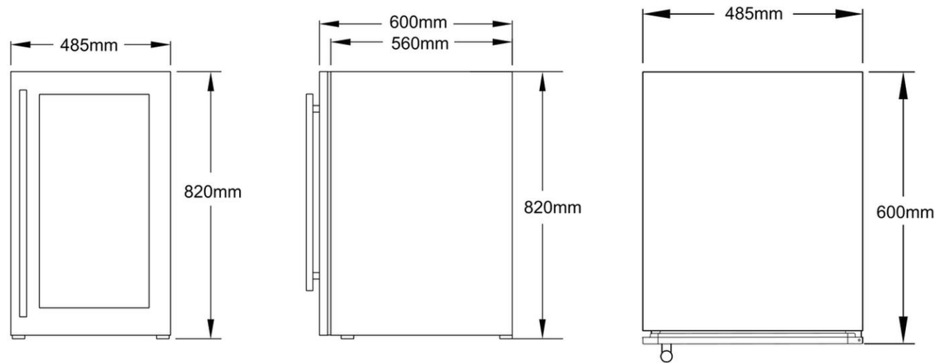
Dimensions — front, side & top
