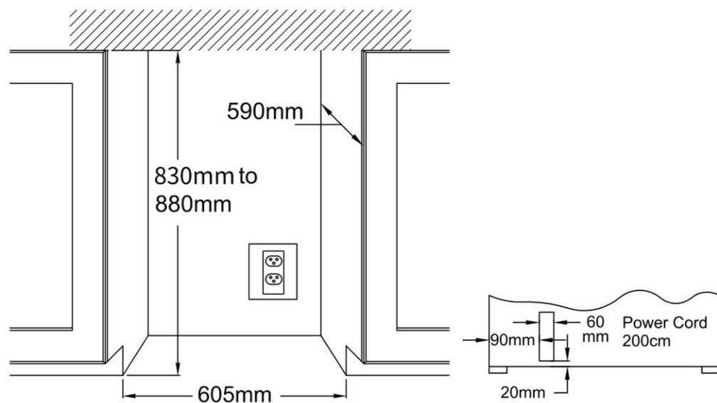
Cabinet Cut-Out
