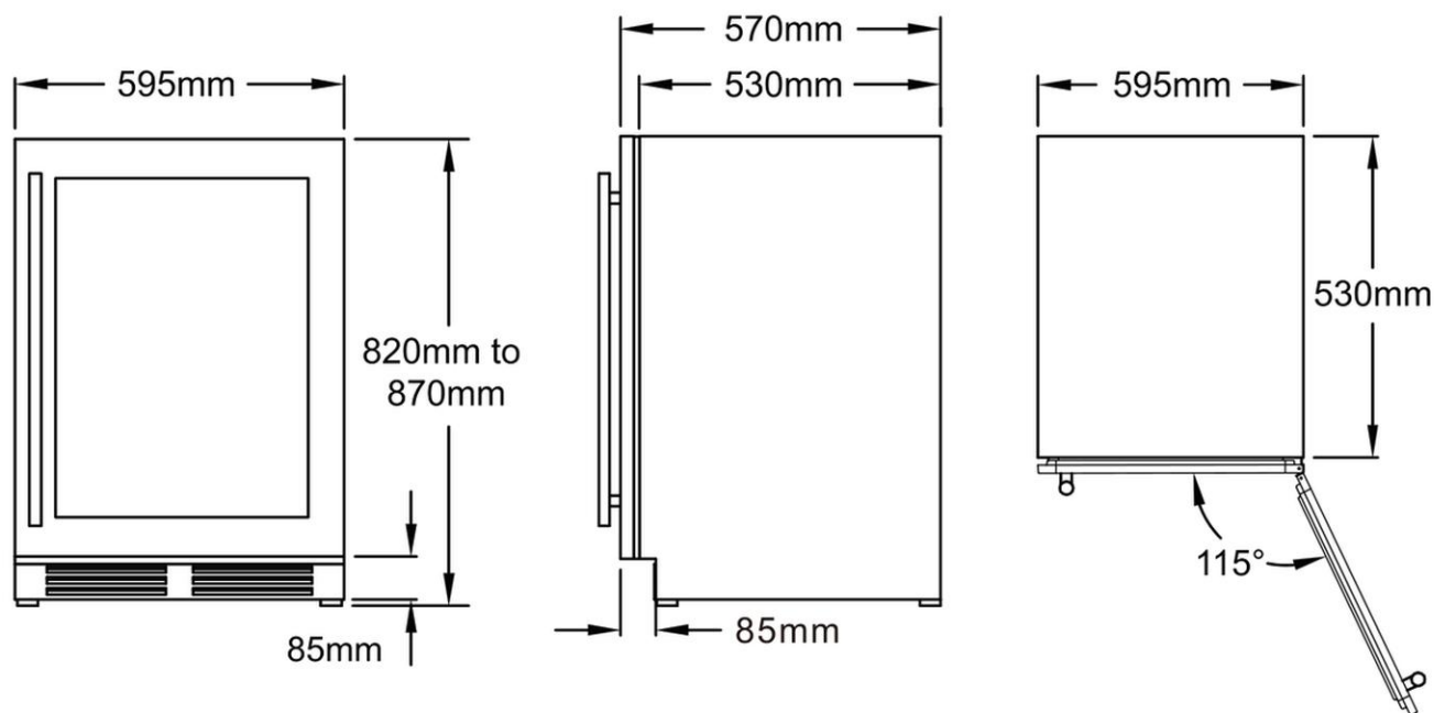
Dimensions — front, side & top
