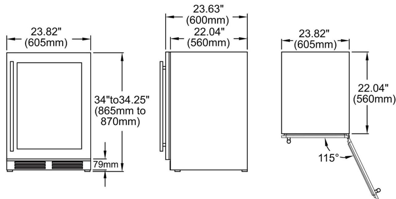
Dimensions — front, side & top
