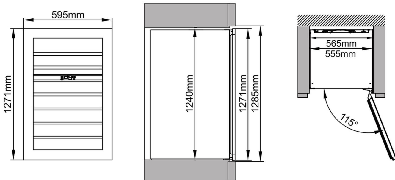
Dimensions — front, side & top
