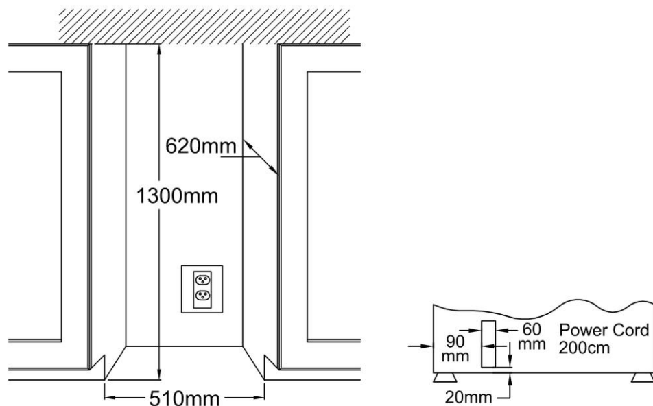
Cabinet Cut-Out
