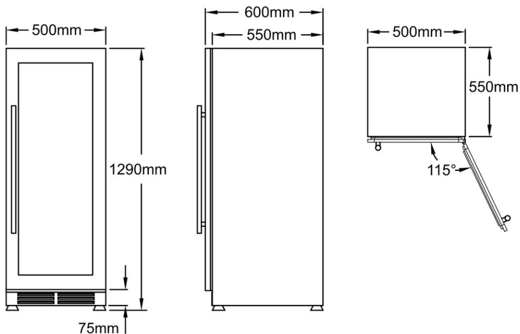
Dimensions — front, side & top
